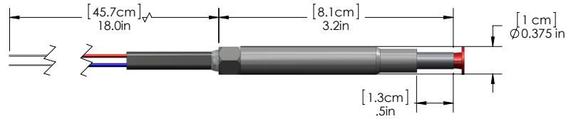
DET-3050-001 Recommended Application: Any Exposed 80 gr. Det Cord
