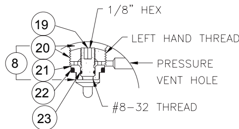
BLEEDER VALVE ASSY. SET-1687-025
