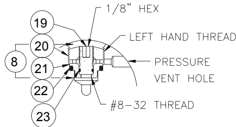
BLEEDER VALVE ASSY. SET-1687-025
